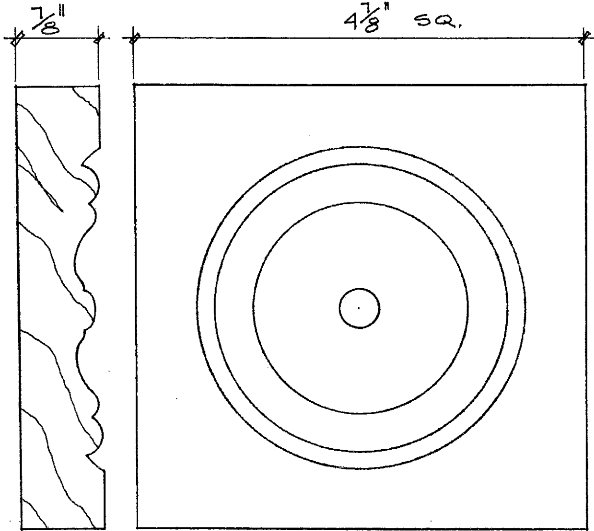
CB-1 7/8" THICKNESS 4 7/8" SQUARE
