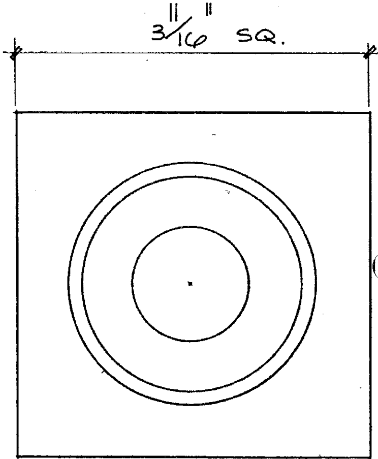
CB-15 7/8" THICKNESS 3 11/16" SQUARE
