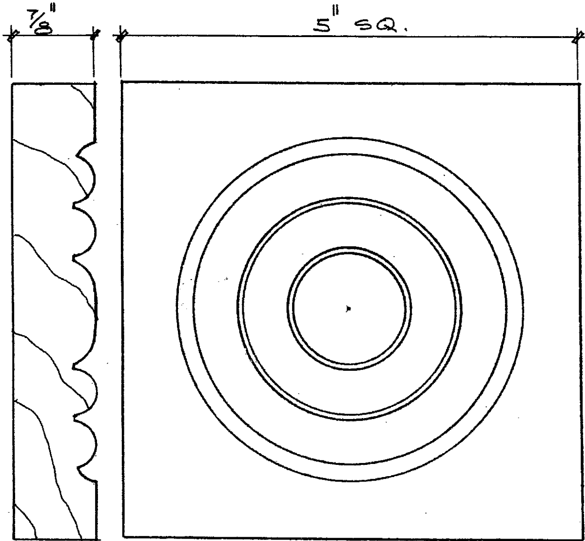
CB-15A 7/8" THICKNESS 5" SQUARE
