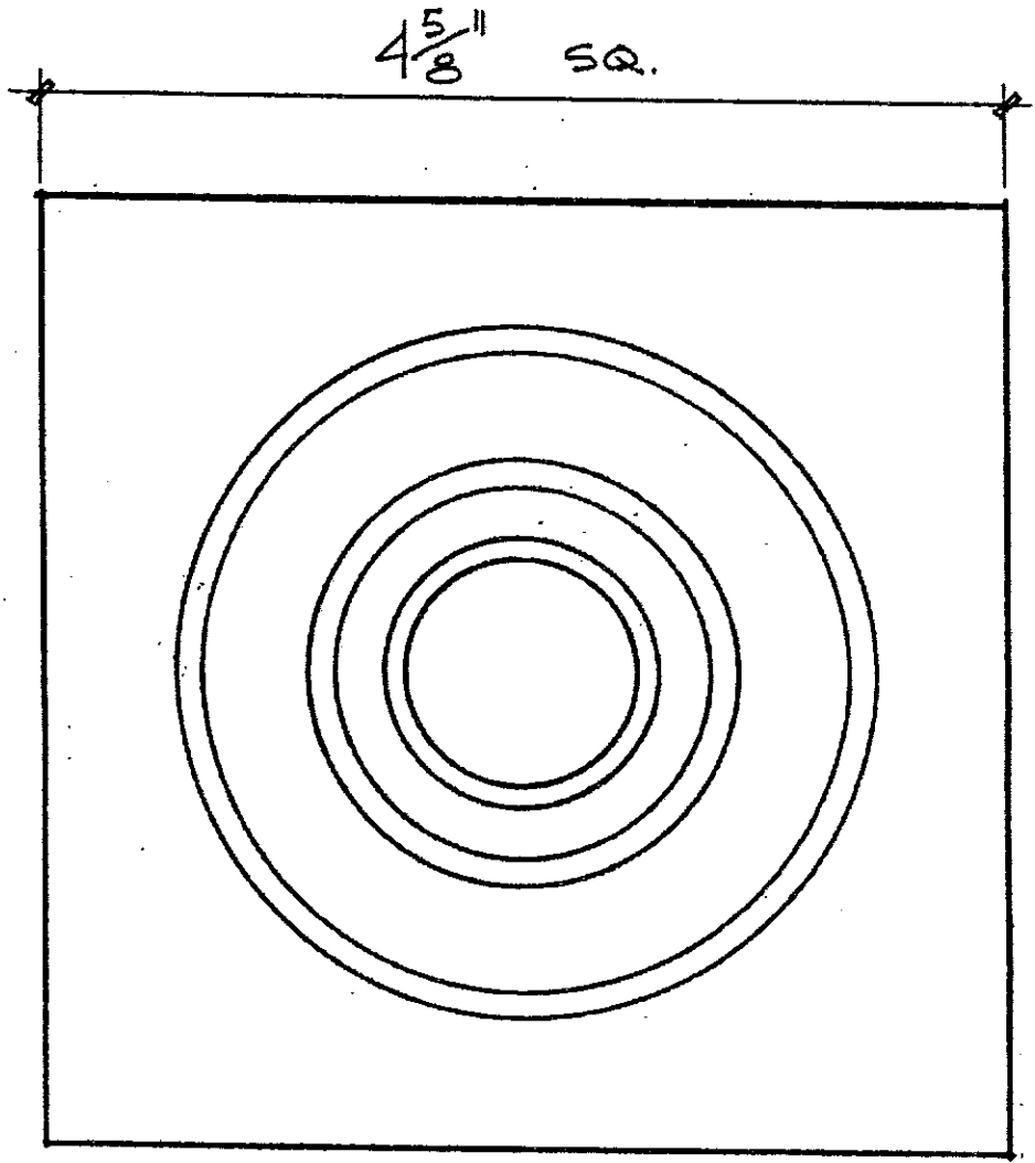
CB-2 7/8" THICKNESS 4 5/8" SQUARE
