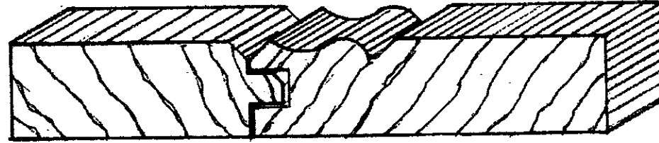
B&S P-14 (9 1/4") 3/4"x9 1/4"
