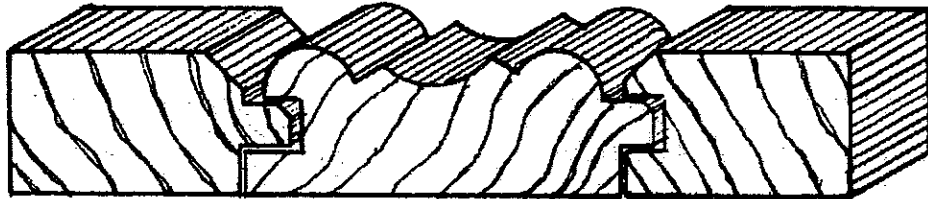
B&S P-4 3/4" x 2 1/4"
