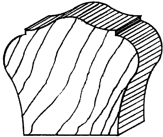
B&S R-2 2 3/16" x 2 1/2"
