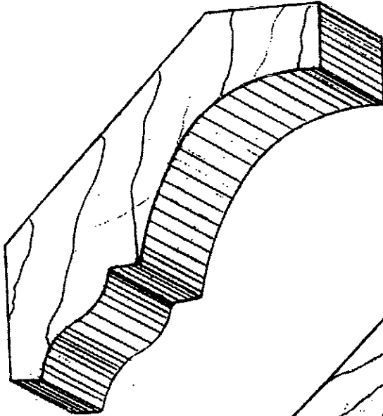
B&S C- 7 13/16"x3 5/8" Drop: 2 13/16" Projection: 2 3/8"
