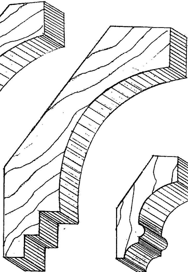
B&S C- 11 1 3/8"x5 3/4" Drop: 4 3/4" Projection: 3 3/8"
