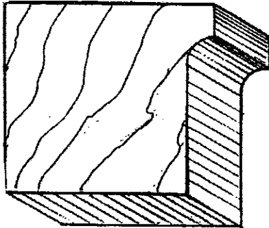
B&S C- 23 1 5/8"x1 1/2" Drop: 1 1/2" Projection: 1 5/8"
