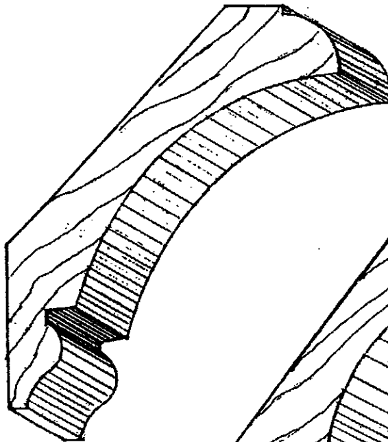
B&S C- 8 1"x3 7/8" Drop: 3 1/8" Projection: 2 5/8"
