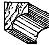
B&S C- 25 7/16"x1/2" Drop: 7/16" Projection: 1/2"
