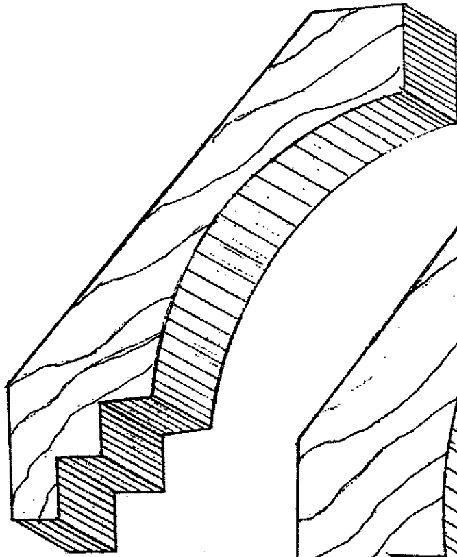
B&S C- 10 7/8"x5" Drop: 3 15/16" Projection: 3 1/8"
