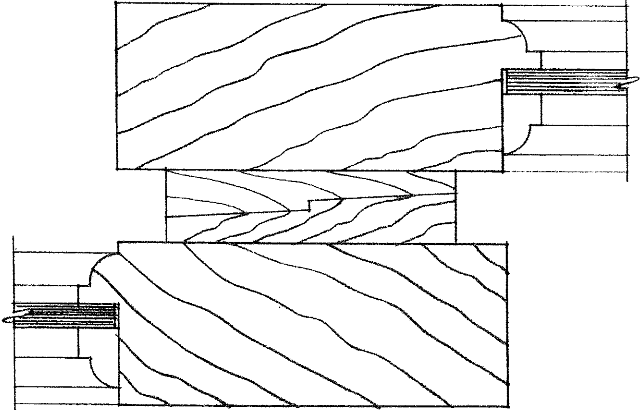
SHOWN: WEATHER STOPS FOR EXTERIOR SLIDING / POCKETING DOORS
