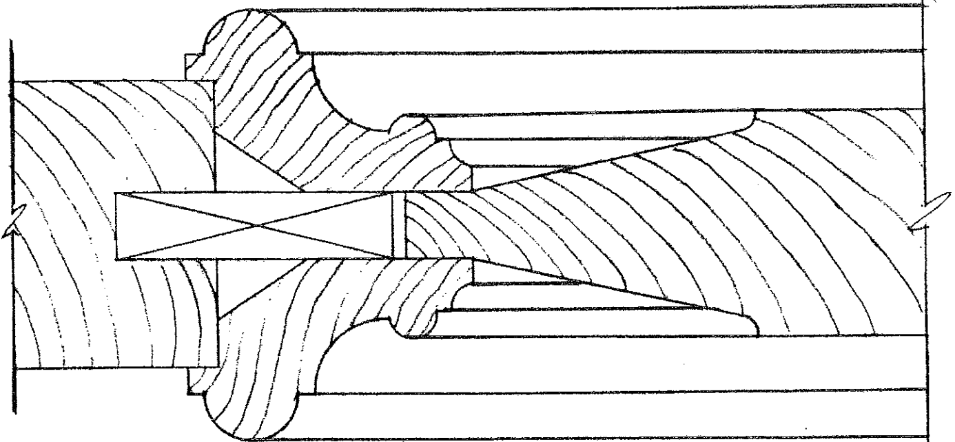
B&S M-128 (1 3/8" x 2 1/8") LIPPED MOULDING; 2 1/4" THICK DOOR; 1 3/4" THICK RAISED PANEL
