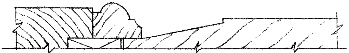
B&S M-133 (5/8" x 7/8") INSET MOULDING; PARTIAL RAISED PANEL
