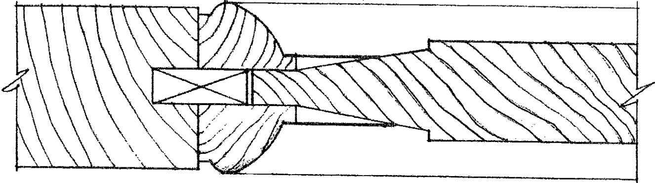
B&S M-136 (3/4" x 1 1/16") INSET MOULDING; 1 3/4" THICK DOOR; 1 1/16" THICK RAISED PANEL
