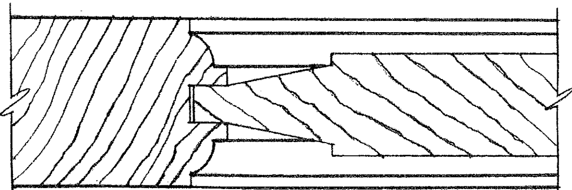
1 3/4" THICK DOOR; 1 1/16" THICK RAISED PANEL
