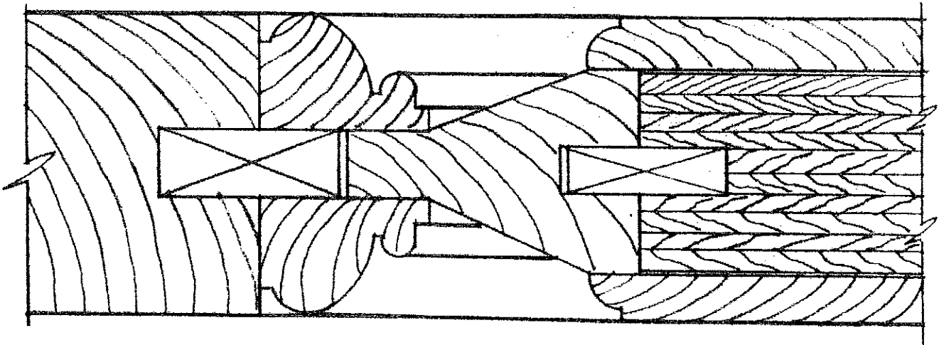
B&S M-126 (7/8" x 1 1/4") INSET MOULDING; 2 1/4" THICK DOOR; 2 1/4" THICK FACE LAMINATED SOLID PANEL
