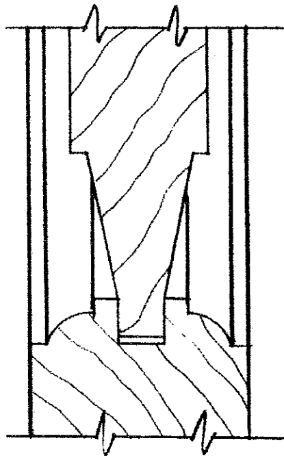
1 3/4" THICK DOOR 1 1/16" THICK RAISED PANEL
