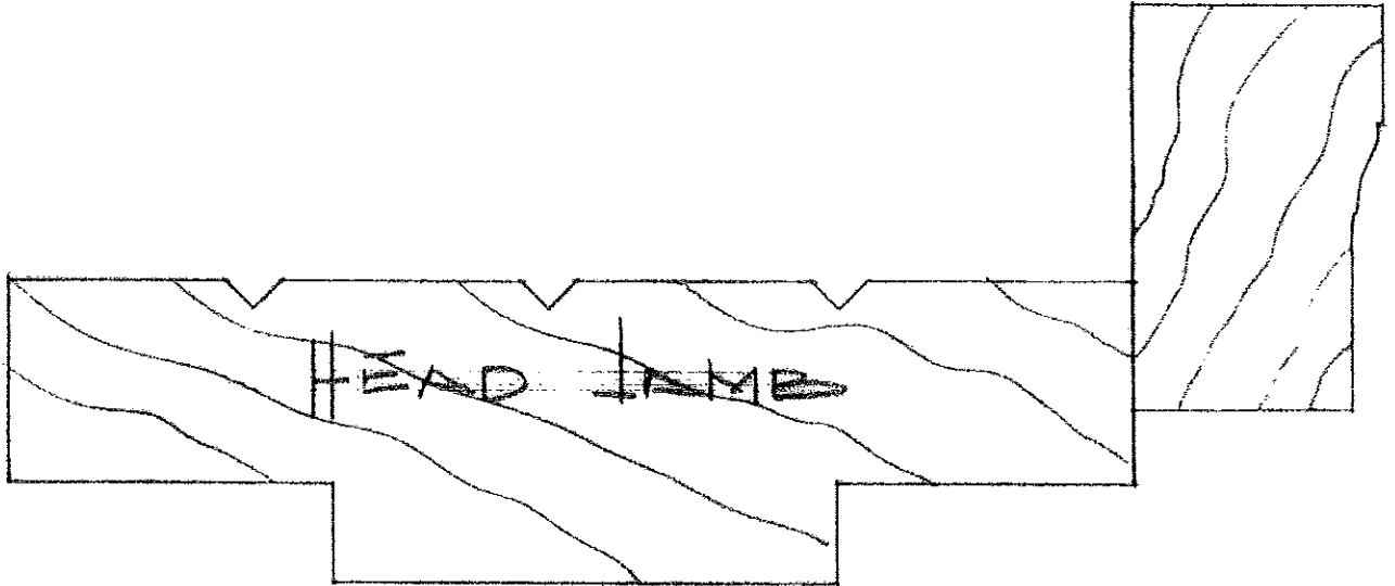
2X6 DOUBLE-RABBETED EXTERIOR DOOR FRAME WM-180 (1 1/4"X2") BRICK MOULDING
