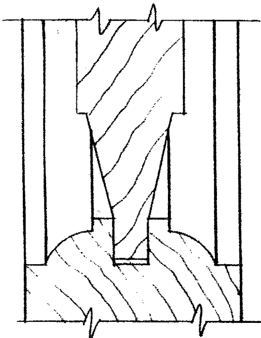
2 1/4" THICK DOOR 1 1/16" THICK RAISED PANEL
