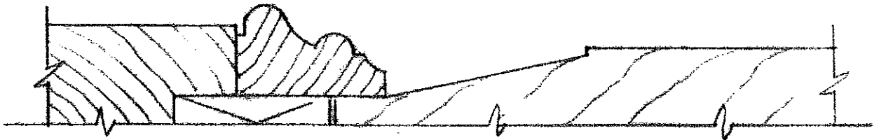
B&S M-131 (11/16" x 1 1/8") INSET MOULDING; PARTIAL RAISED PANEL
