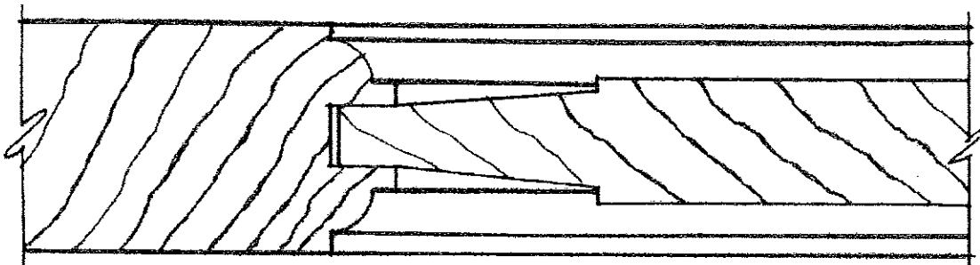
1 3/8" THICK DOOR; 3/4" THICK RAISED PANEL
