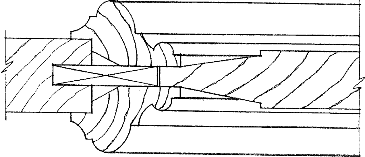
B&S M-121 (1 3/16" x 2") LIPPED MOULDING; 1 3/8" THICK DOOR; 1 1/16" THICK RAISED PANEL
