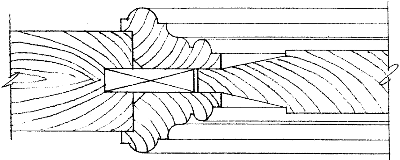
B&S M-129 (1 1/16"X1 11/16") LIPPED MOULDING; 1 3/4" THICK DOOR; 1 1/16" THICK RAISED PANEL
