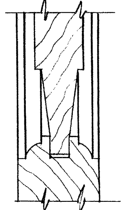
1 3/8" THICK DOOR 3/4" THICK RAISED PANEL
