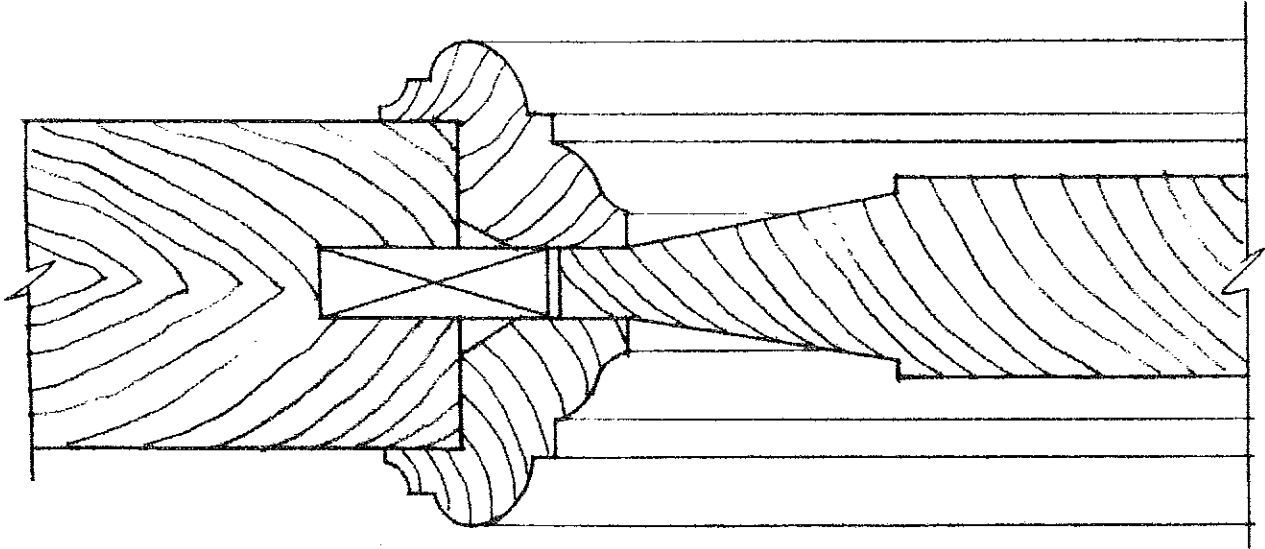
B&S M-127 (1 1/8" x 1 1/4") LIPPED MOULDING; 1 3/4" THICK DOOR; 1 1/16" THICK RAISED PANEL
