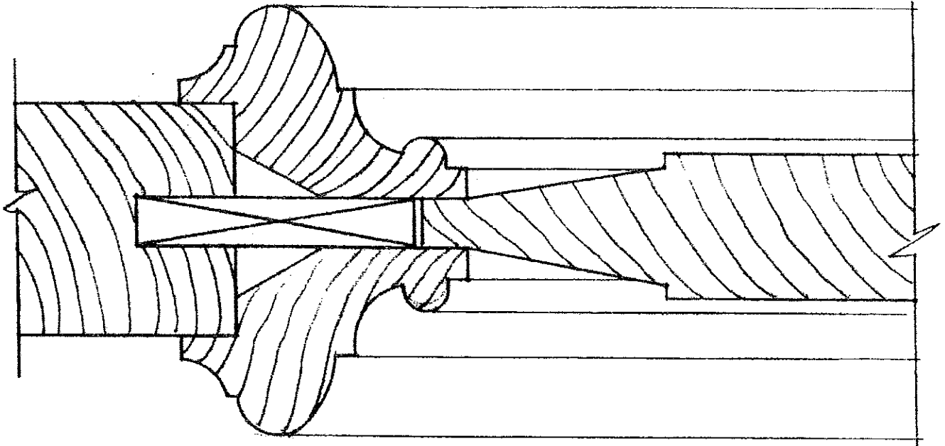
B&S M-122 (1 3/8" x 2 1/8") LIPPED MOULDING; 1 3/4" THICK DOOR; 1 1/16" THICK RAISED PANEL
