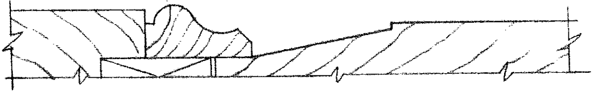
B&S M-130 (9/16" x 1 1/8") INSET MOULDING; PARTIAL RAISED PANEL
